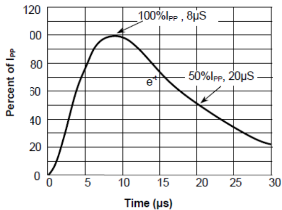
Fig.3 Pulse Waveform-8/20μs
